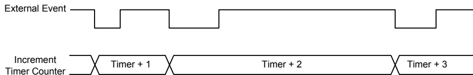
Event Counter Mode Timing Chart (T0EG=1)
