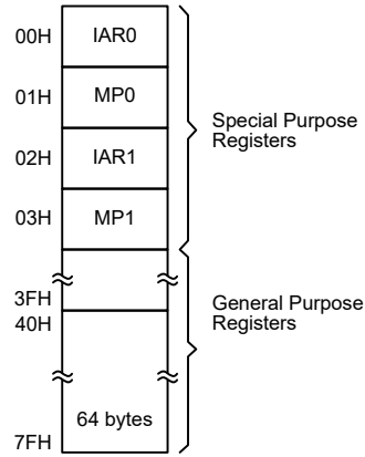
Data Memory Structure
