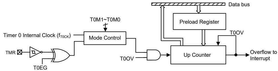
8-bit Timer/Event Counter 0 Structure
