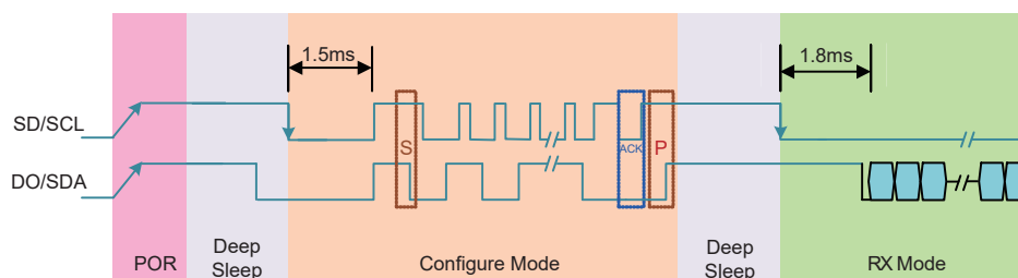
Entering and Leaving Configuration Mode Timing Diagram
