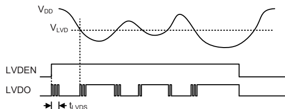
LVD Operation
