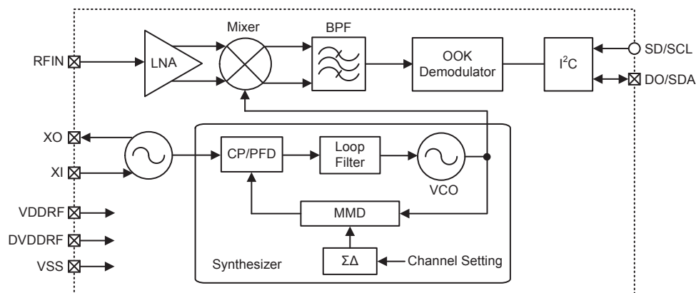
RF Receiver Block Diagram
