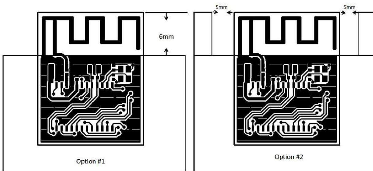
Figure 11 Schematic diagram of the antenna layout
