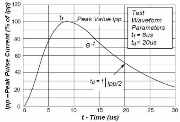
Pulse Waveform
