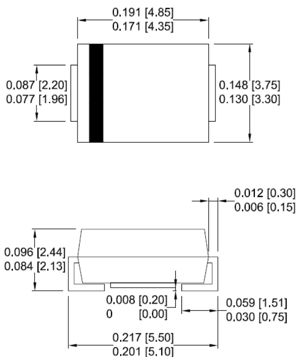
SMB/ DO-214AA
