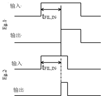
图 8：典型输入滤波 Figure 8: Typical input filtering Figure
