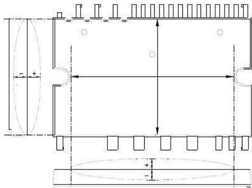
图 7：平面度检测位置 Figure 7: Flatness detection position
