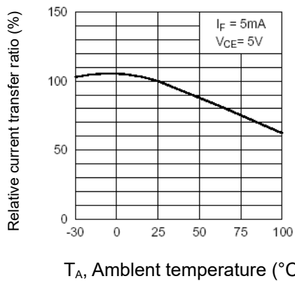
Figure 7: Relative Current Transfer Ratio vs. Ambient Temperature
