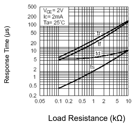
Figure 10: Response Time vs. Load Resistance
