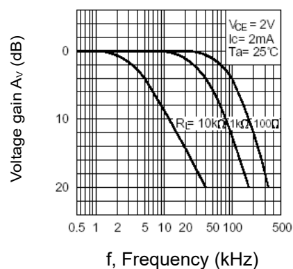
Figure 11: Frequency Response
