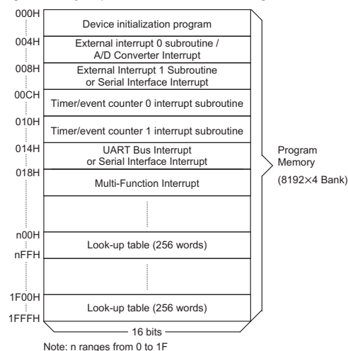
Program Memory
