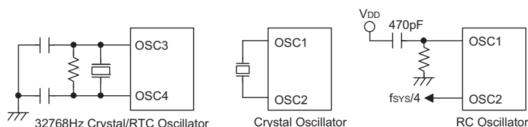
System Oscillator
