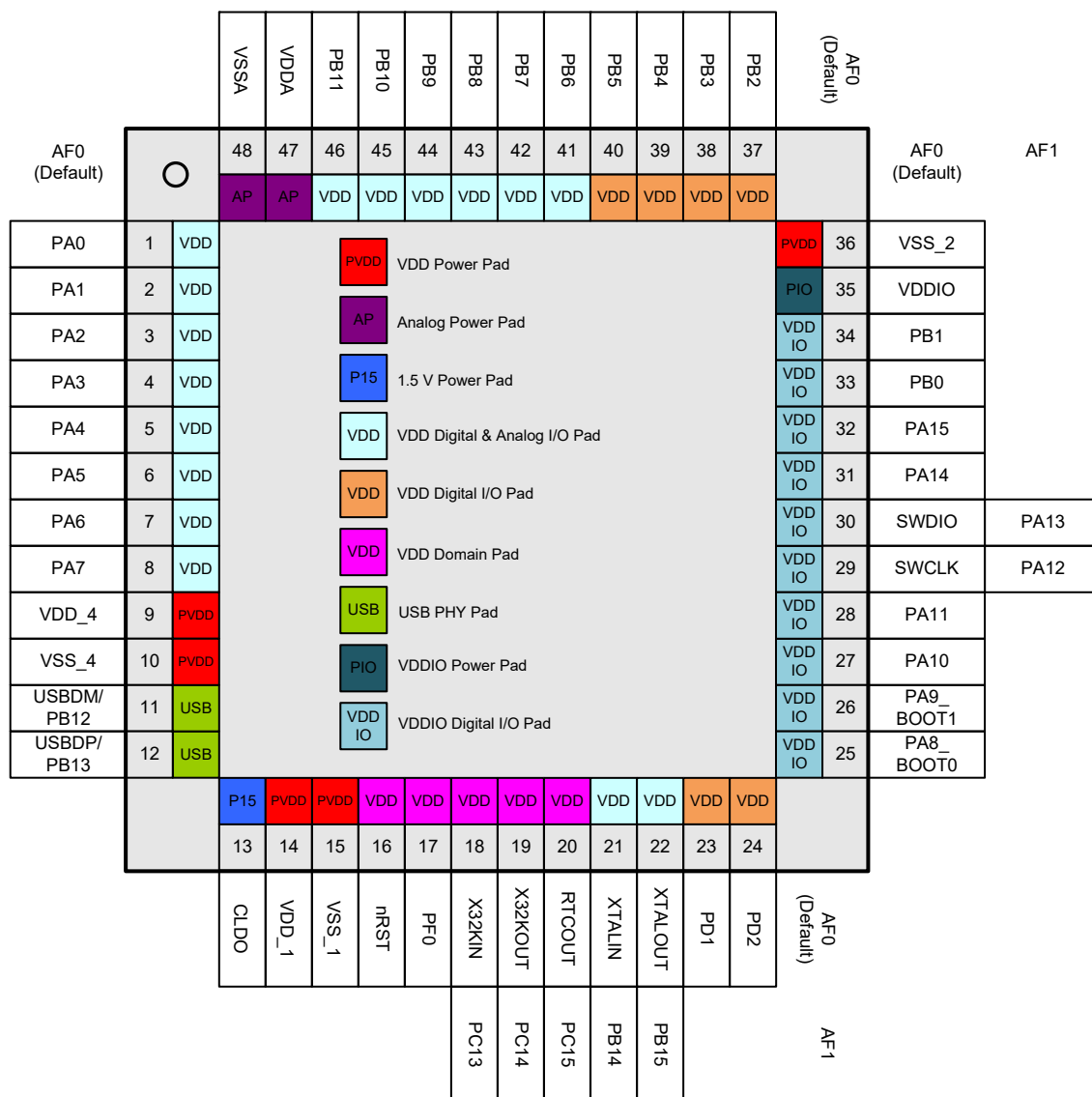
Figure 5. 48-pin LQFP Pin Assignment
