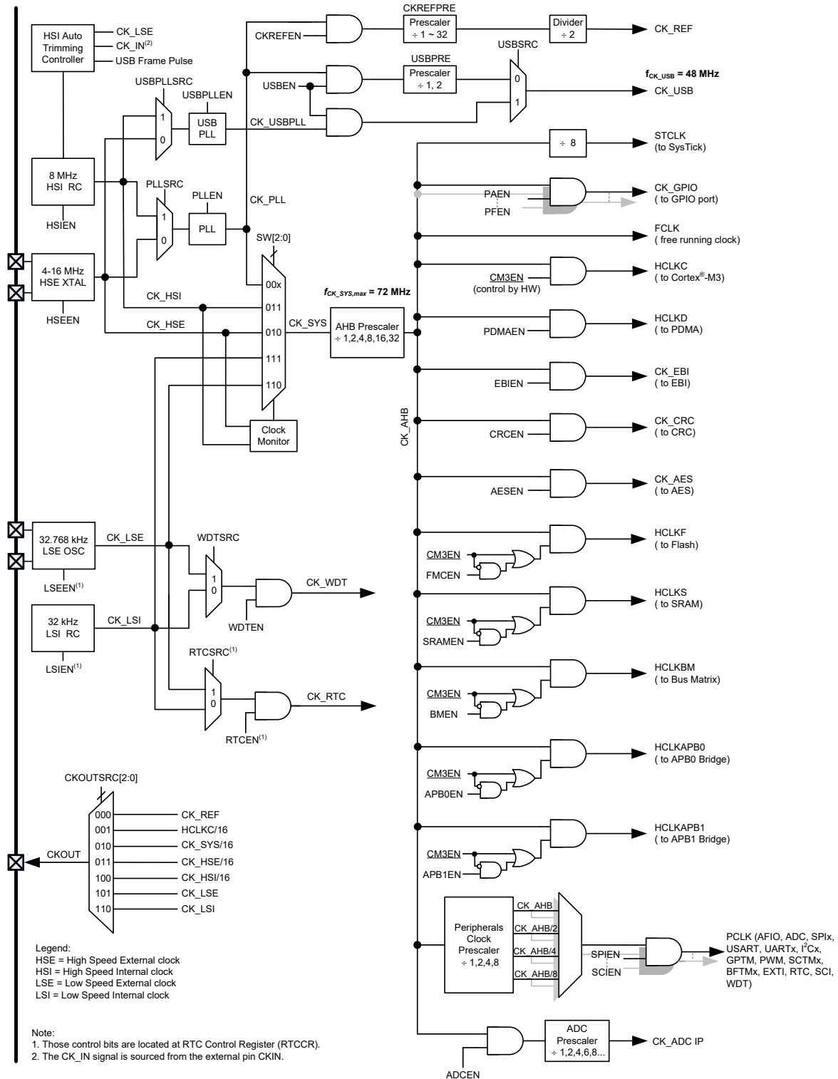
Figure 3. Clock Structure
