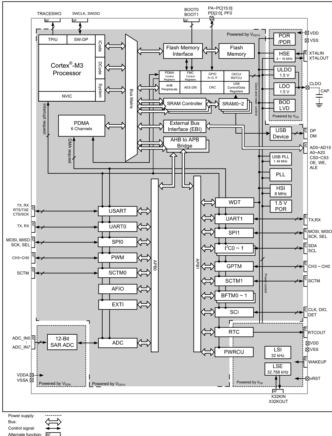
Figure 1. Block Diagram
