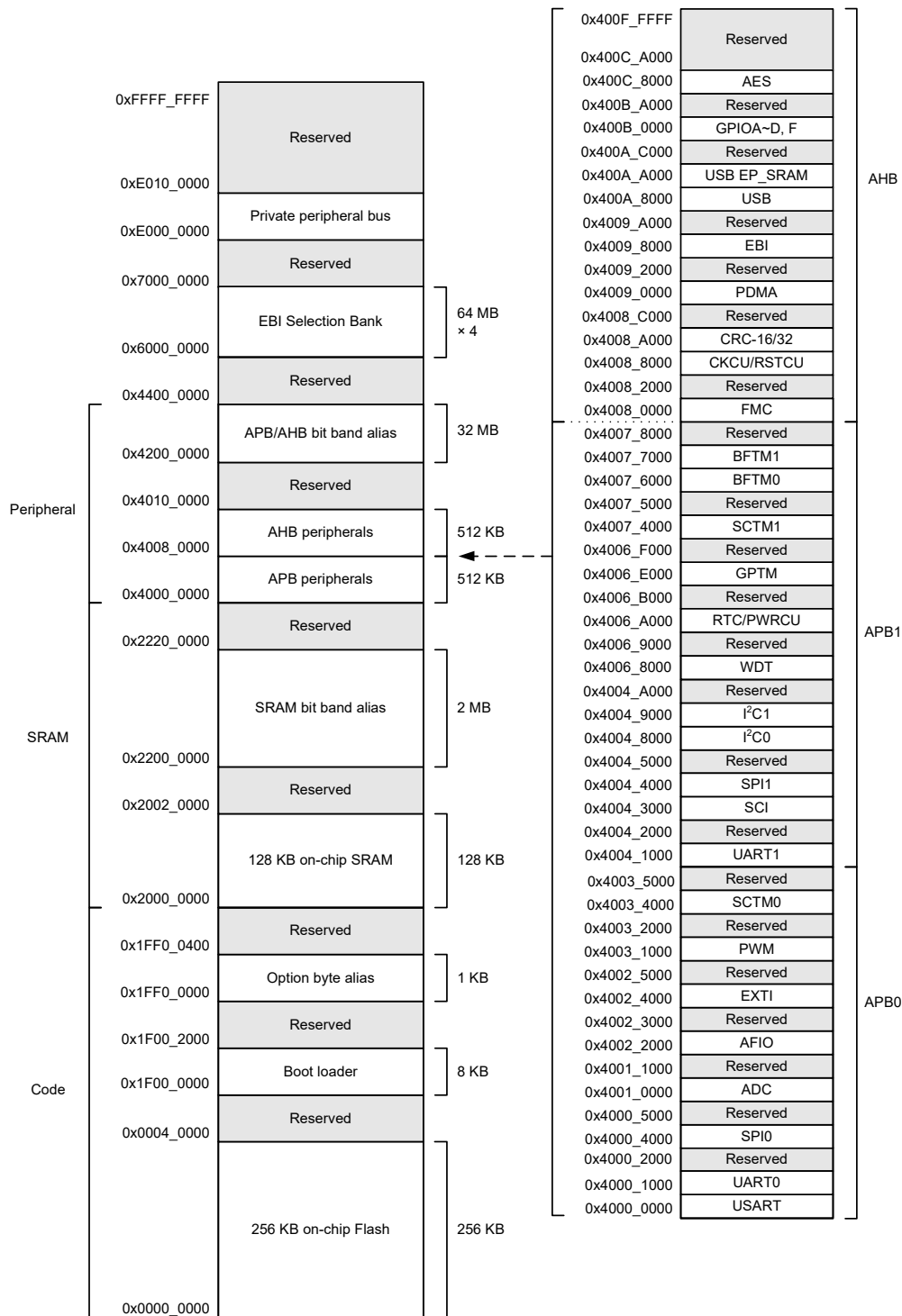
Figure 2. Memory Map
