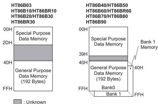
RAM Data Memory Structure – Bank 0, Bank1
