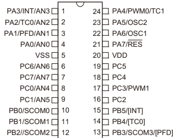
HT46R066 24 SKDIP-A/SOP-A/SSOP-A
