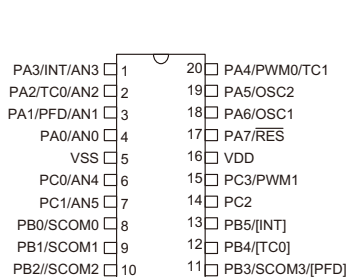
HT46R066 20 DIP-A/SOP-A/SSOP-A
