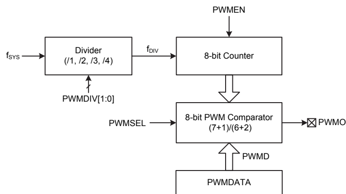
PWM Block Diagram
