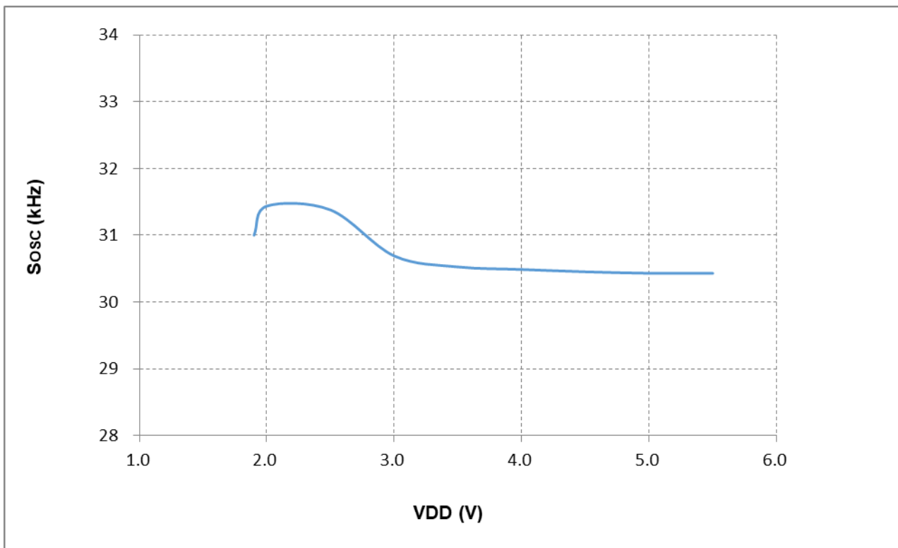
Figure 14-2 LIRC vs. V_{DD} ( T_A = 25^\circ\text{C} )
