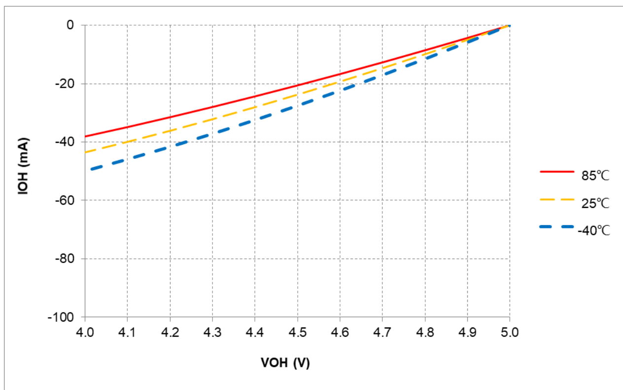
Figure 14-8 I_{OH} vs. V_{OH} @L3 = -24mA , V_{DD} = 5V
