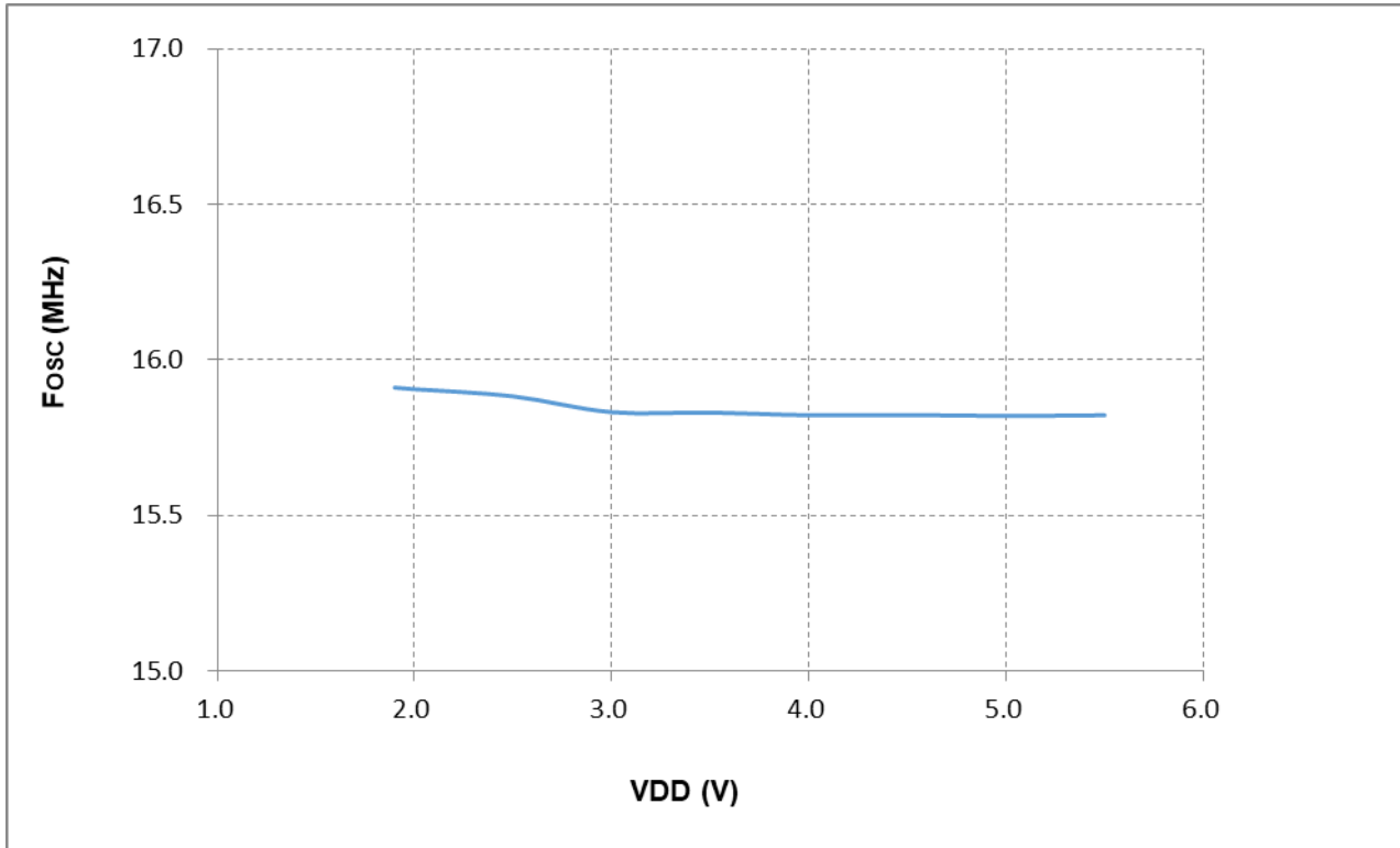
Figure 14-1 HIRC vs. V_{DD} ( T_A = 25^\circ\text{C} )
