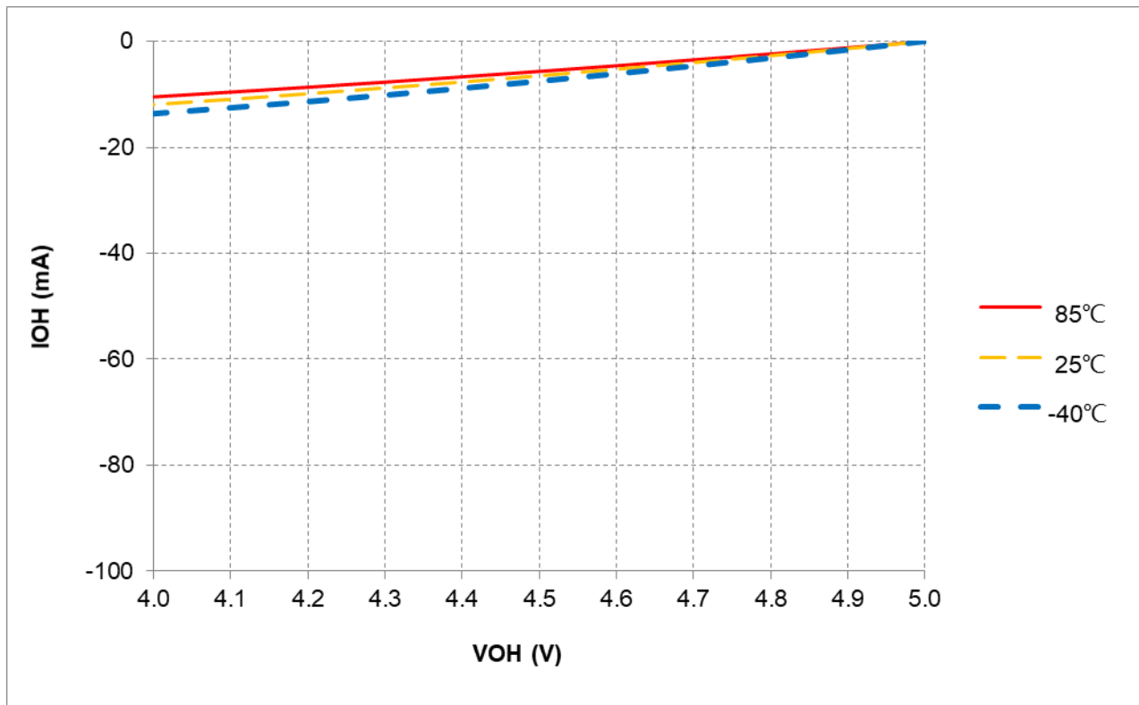
Figure 14-6 I_{OH} vs. V_{OH} @L1 = -6mA , V_{DD} = 5V
