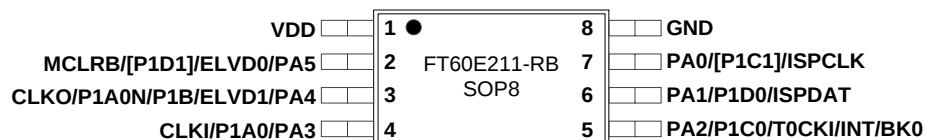
Figure 1-3 SOP8
