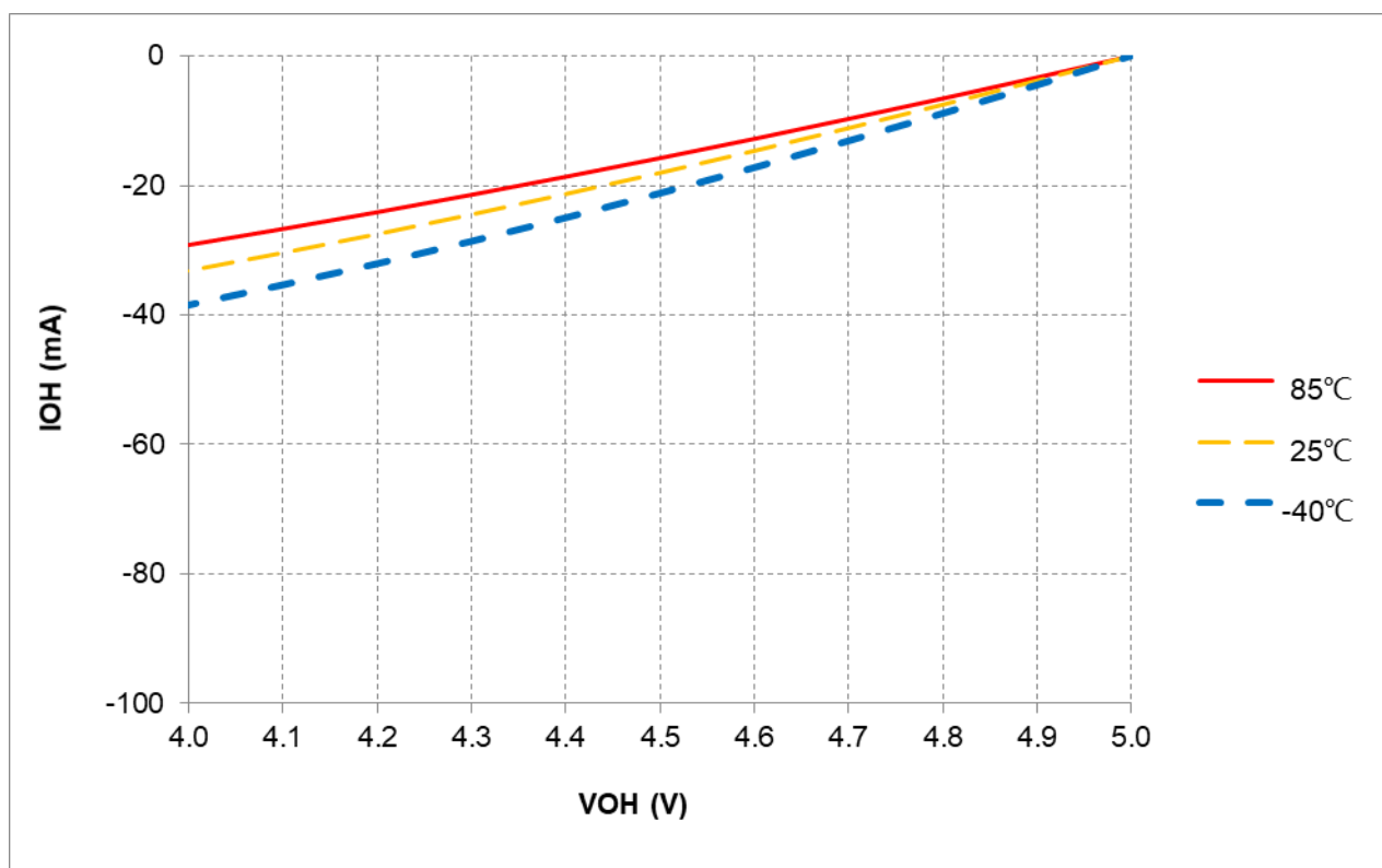
Figure 14-7 I_{OH} vs. V_{OH} @L2 = -18mA , V_{DD} = 5V
