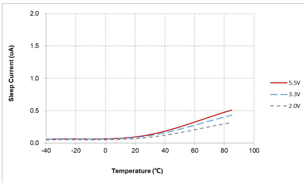
Figure 14-4 Sleep Current ( I_{SB} ) vs. Temperature
