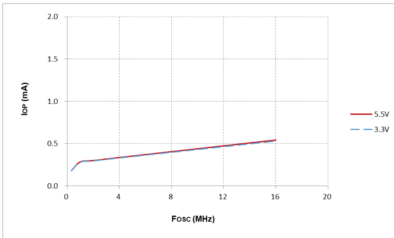
Figure 14-3 I_{DD} vs. Frequency (4T, T_A = 25^\circ\text{C} )
