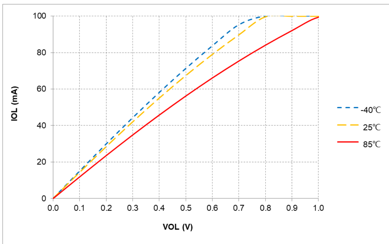
Figure 14-10 I_{OL} vs. V_{OL} @ L1 = 67mA , V_{DD} = 5V
