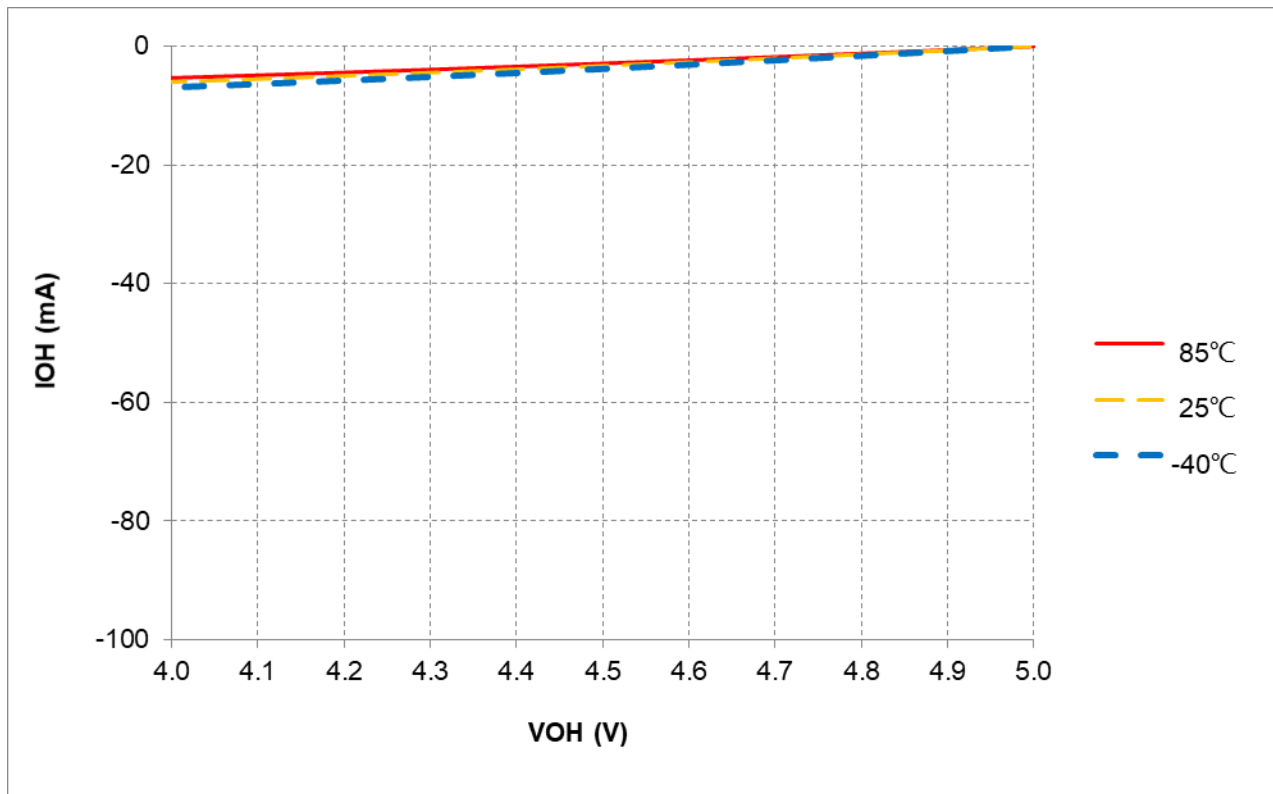
Figure 14-5 I_{OH} vs. V_{OH} @L0 = -3mA , V_{DD} = 5V
