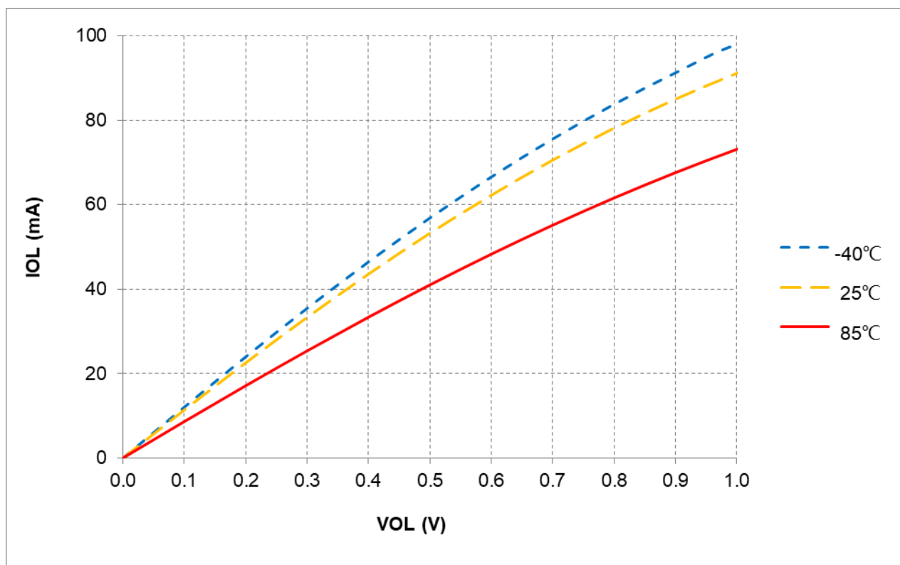
Figure 14-9 I_{OL} vs. V_{OL} @ L0 = 53mA , V_{DD} = 5V
