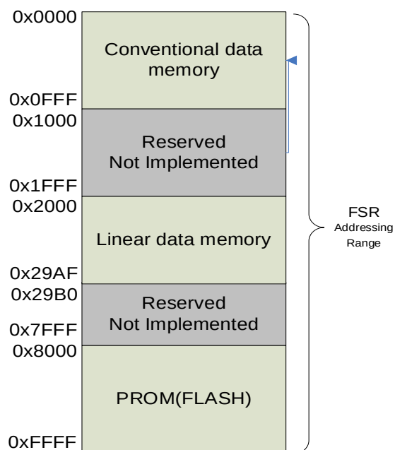
Figure 17-3 Indirect addressing
