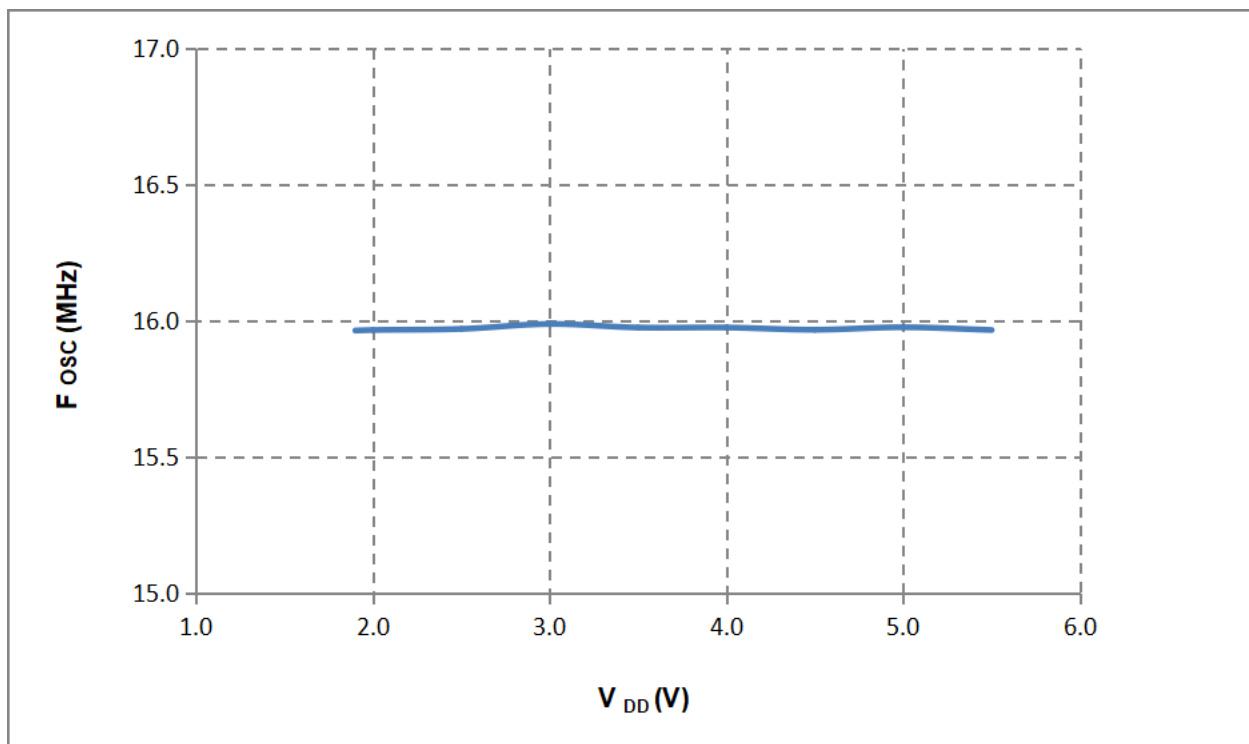
Figure 20-1 HIRC vs. V_{DD} ( T_A = 25^\circ\text{C} )
