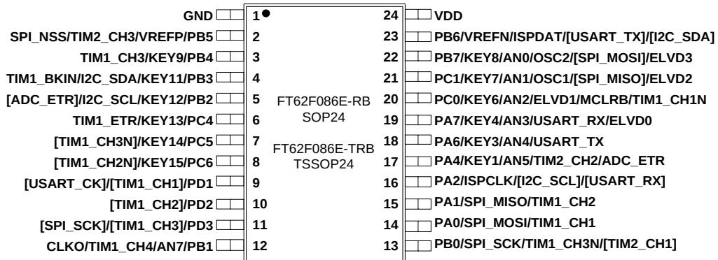
Figure 1-4 SOP24 / TSSOP24
