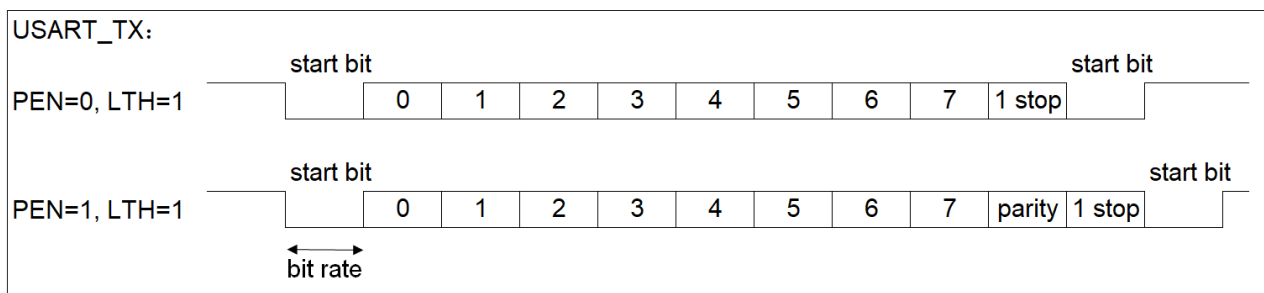
Figure 14-2 Communication Format in Asynchronous Mode (take 8bit length as an example)
