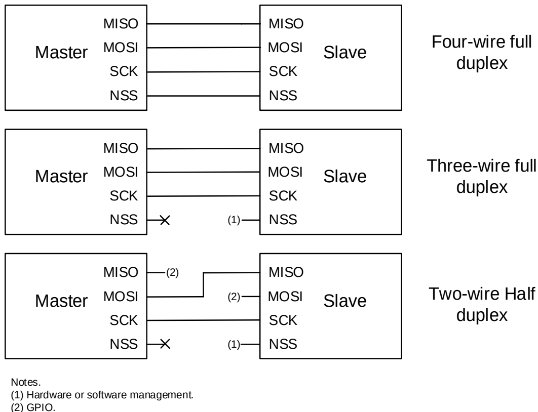
Figure 12-2 Connection Diagram of SPI Interface Pin
