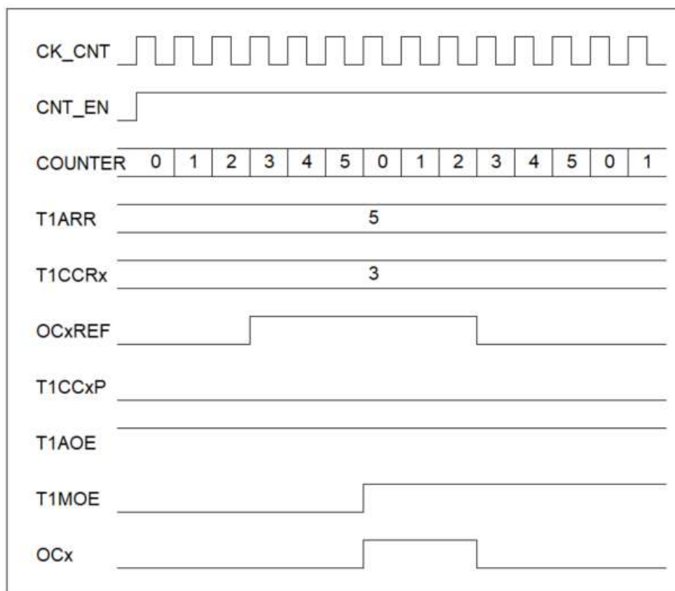
Figure 7-21 Output Timing Diagram when Toggle on Match
