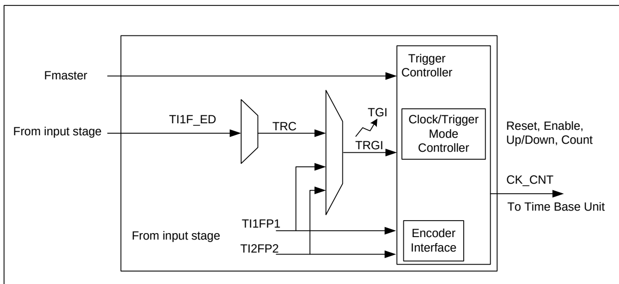
Figure 7-10 Clock/trigger controller Block Diagram
