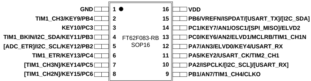
Figure 1-2 SOP16
