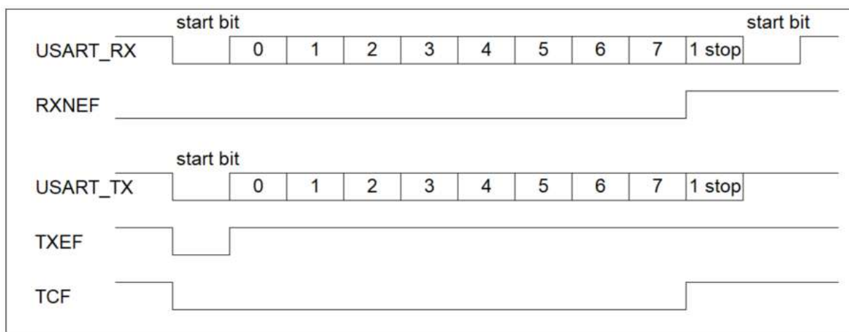
Figure 14-3 Asynchronous Mode Flag Timing Diagram
