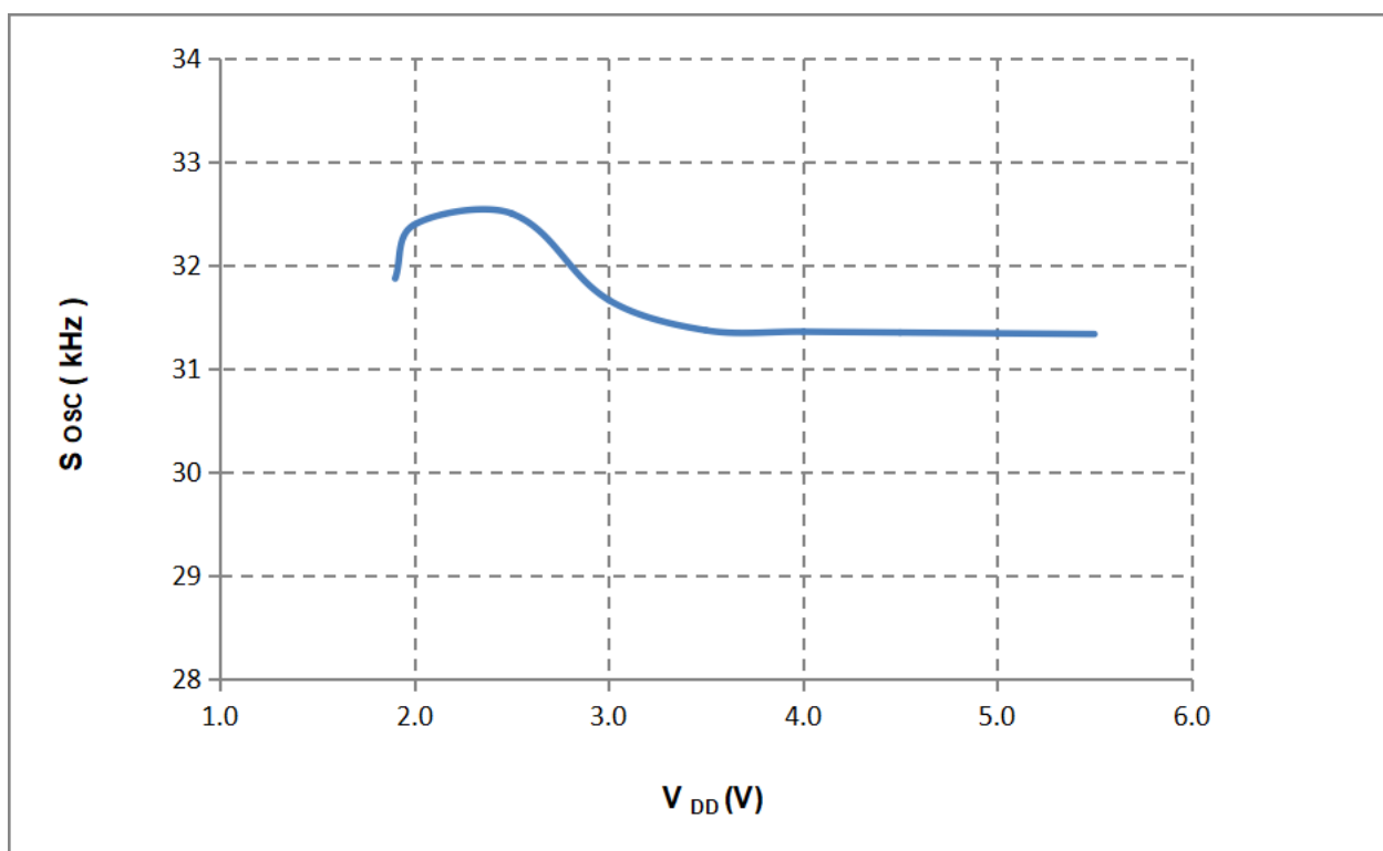
Figure 20-2 LIRC vs. V_{DD} ( T_A = 25^\circ\text{C} )
