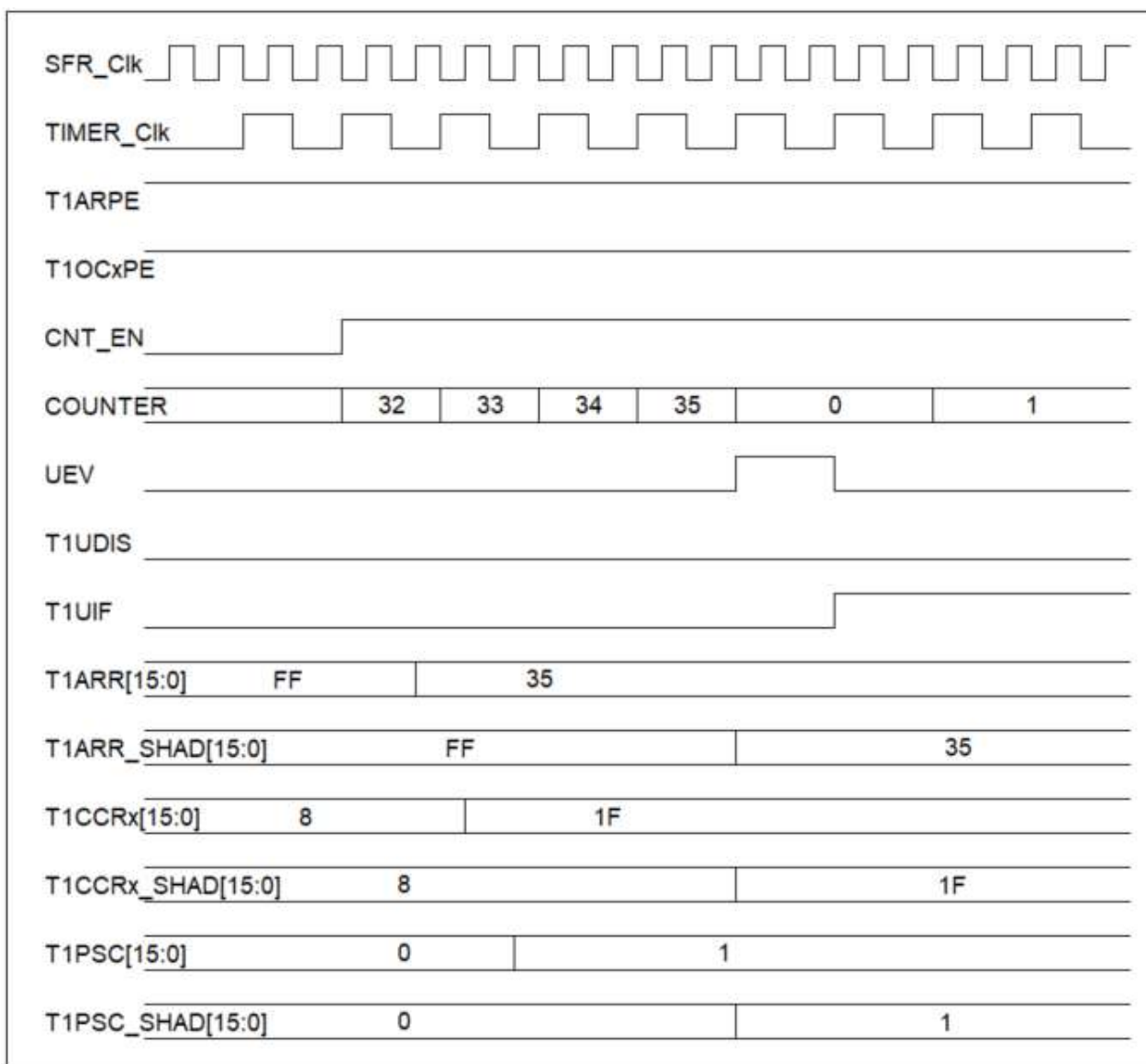
Figure 7-4 Update timing diagram of the preload register under update event
