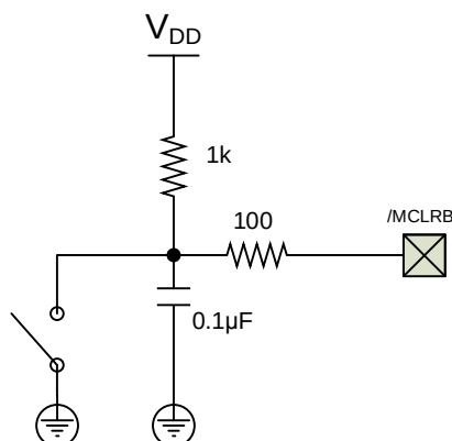
Figure 4-3 /MCLR reset circuit
