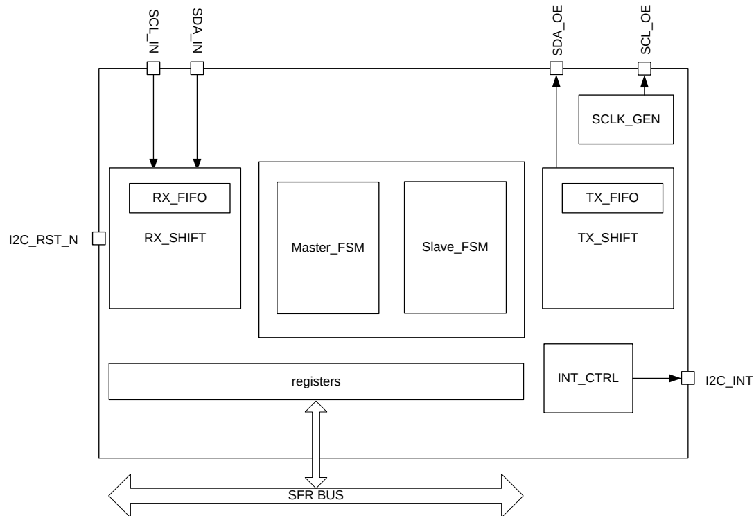
Figure 13-1 I2C Block Diagram
