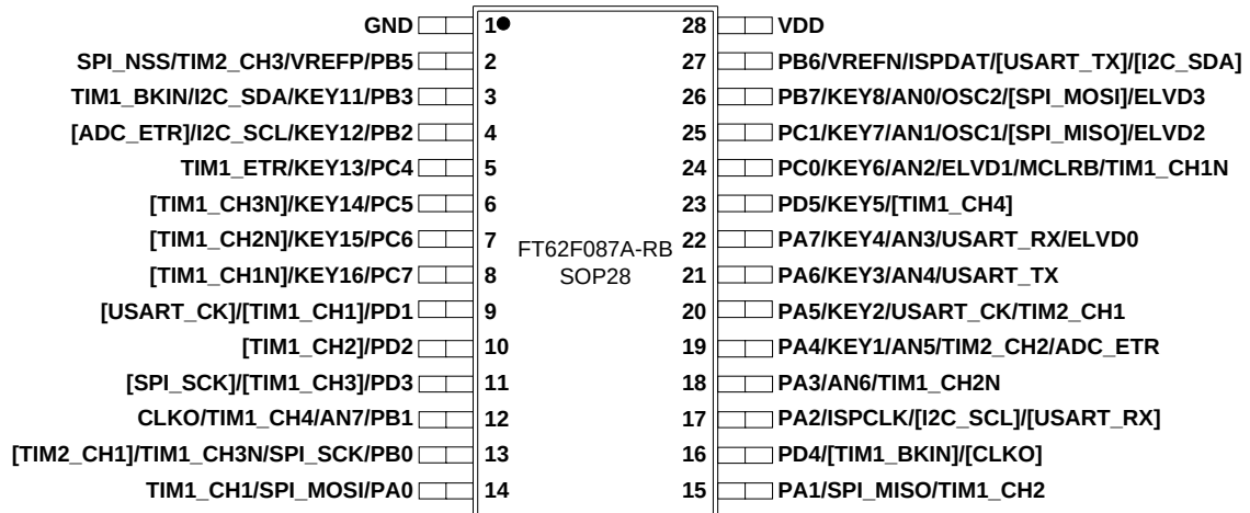
Figure 1-5 SOP28 (A) 1
