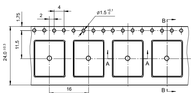
Tape Dimensions (Short terminal SMT)
