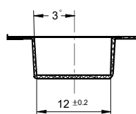
Tape Dimensions (Short terminal SMT)
