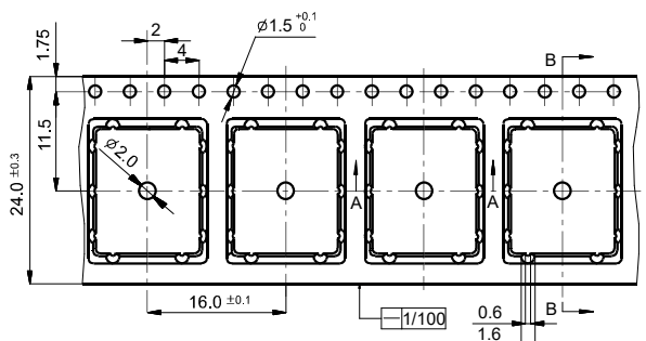
Tape Dimensions (Short terminal SMT)
