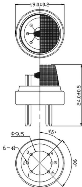
figure 1 Sensing Structure Diagram
