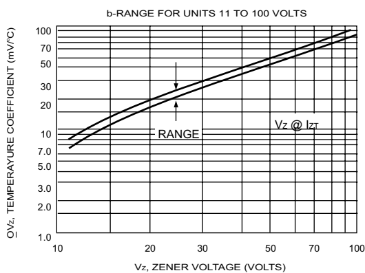
FIG.8- TEMPERATURE COEFFICIENTS
