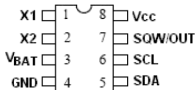
DIP-8/SOP-8/MSOP-8
