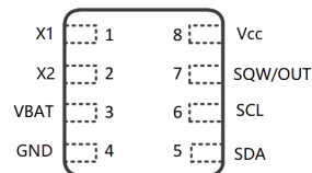
DFN-8 3*3
